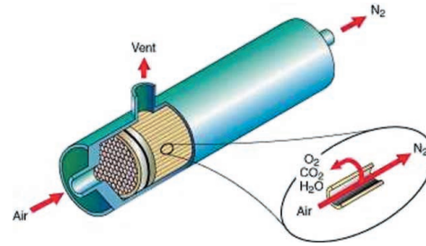
Nitrogen is produced from compressed air
